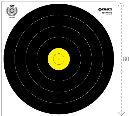
Name : FIELD 80cm Target Face [PT 014] Mark dimension : 80cmX80cm Target Total dimension : 83cmX83cm(width/length)
